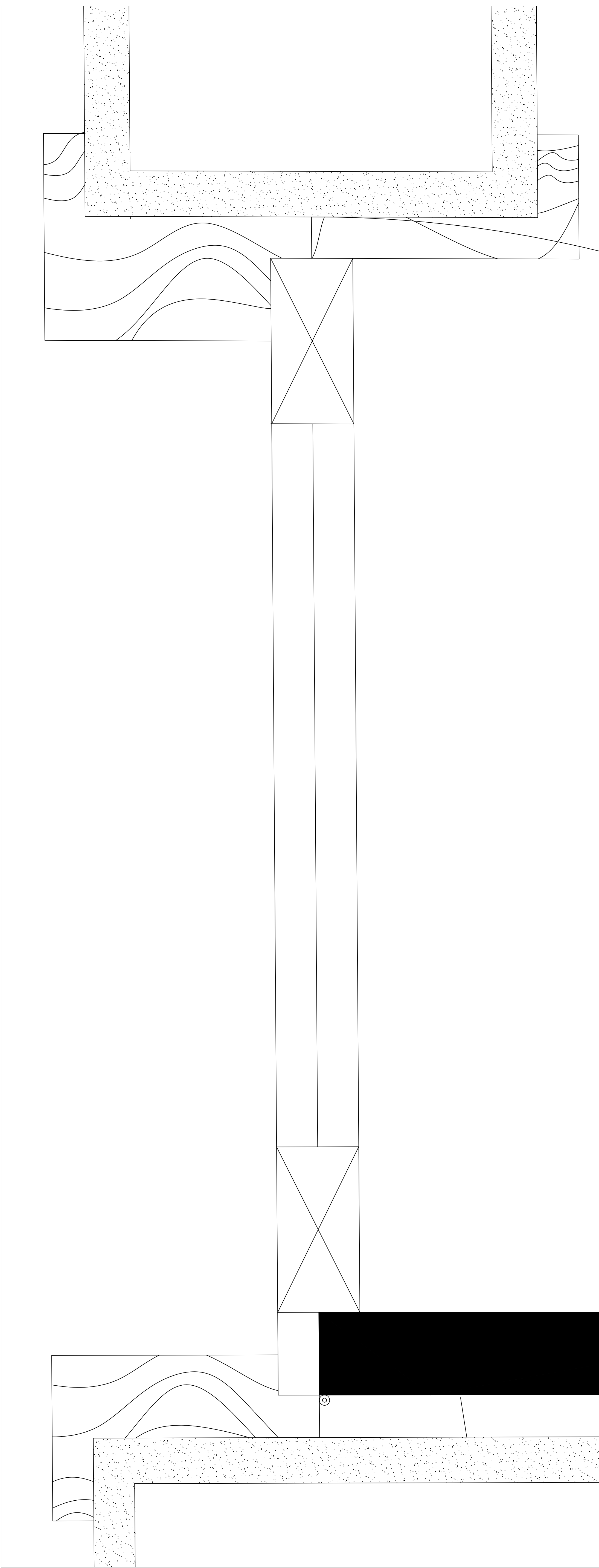
Pormenor porta 1:1
